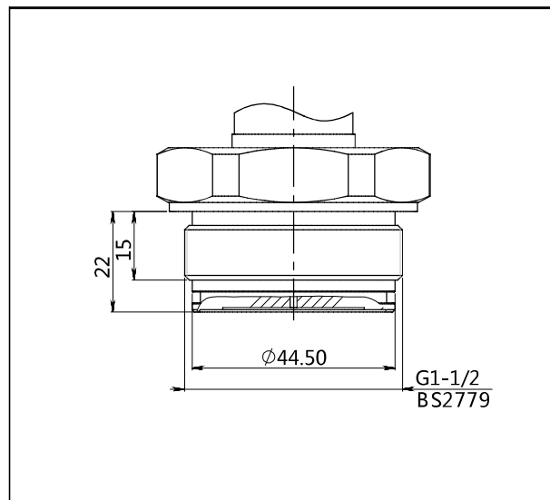
Process connection(G07) (unit: mm)
