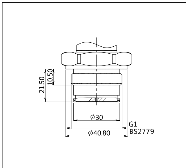
Process connection(K-1) (unit: mm)
