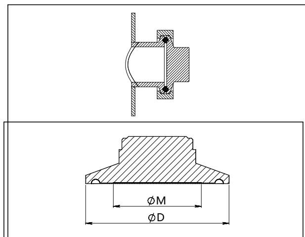
Process connection(K-1) (unit: mm)
