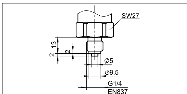
Process connection(R) (unit: mm)
