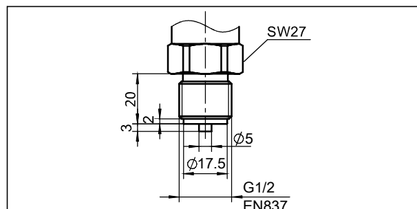
Process connection(G) (unit: mm)
