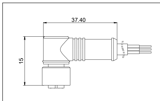
Aviation female plug elbow(Z2) (unit: mm)
