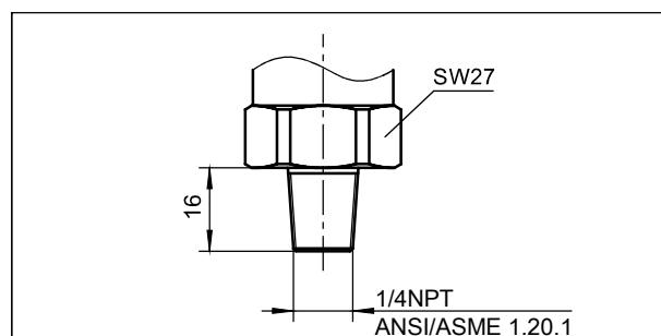
Process connection(R2) (unit: mm)
