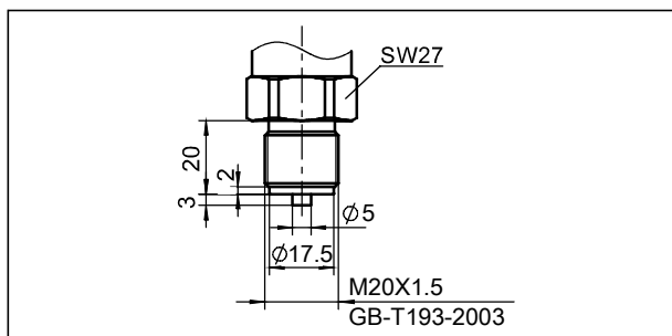
Process connection(G2) (unit: mm)
