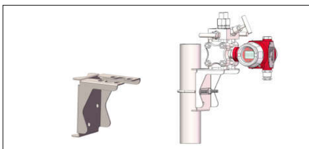
Pipe mounting bent bracket(B1)
